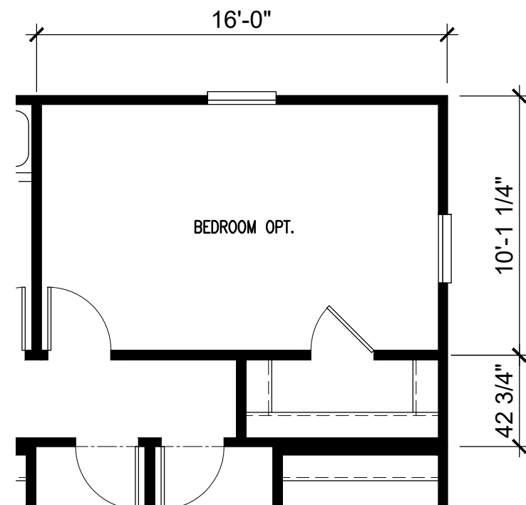
BEDROOM 4 OPTION
