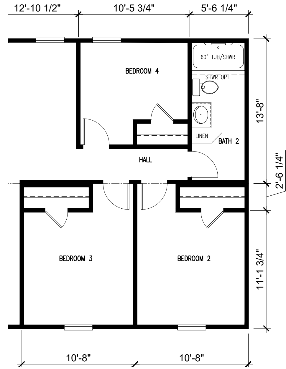
BEDROOM 4 OPTION
